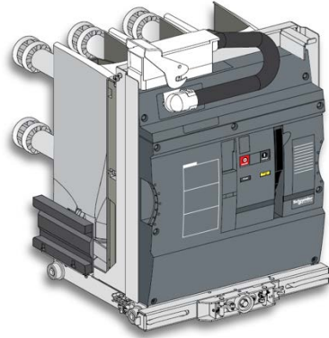
EasyPact 12kV Tipe Withdrawable
