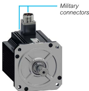
130 mm/5.12 in
