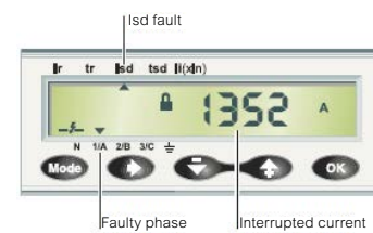
Display of interrupted current.
